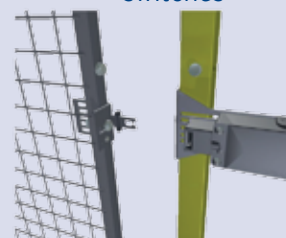
Universal holder for the installation of actuators and micro-switches
